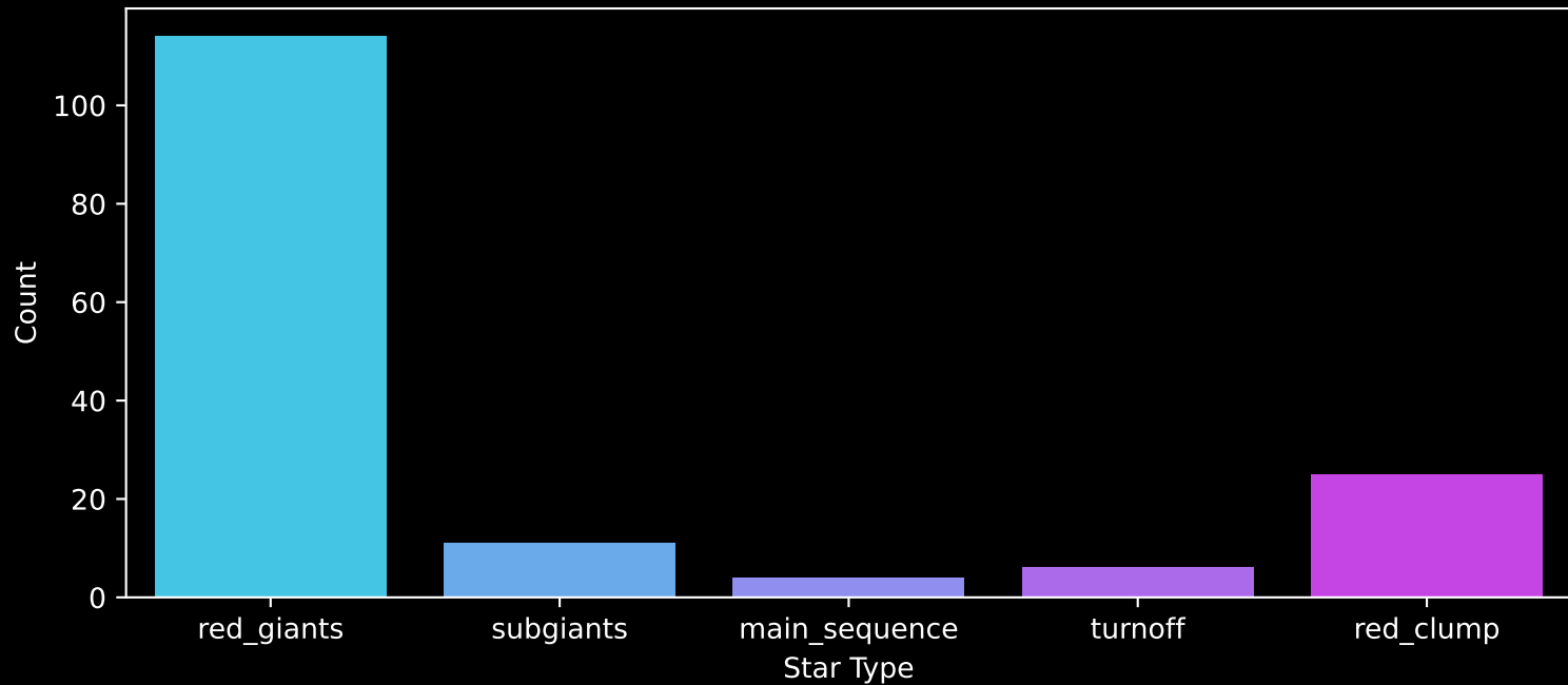
APOGEE DR17 Field: [229+04] Count plot of Star Type
