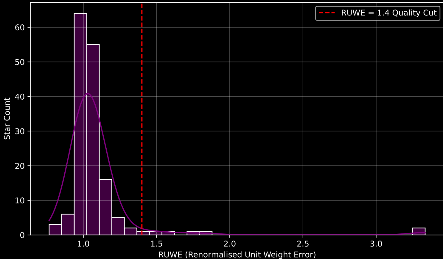
GAPOGEE DR17 Field [229+04] RUWE Distribution (n= 158)
