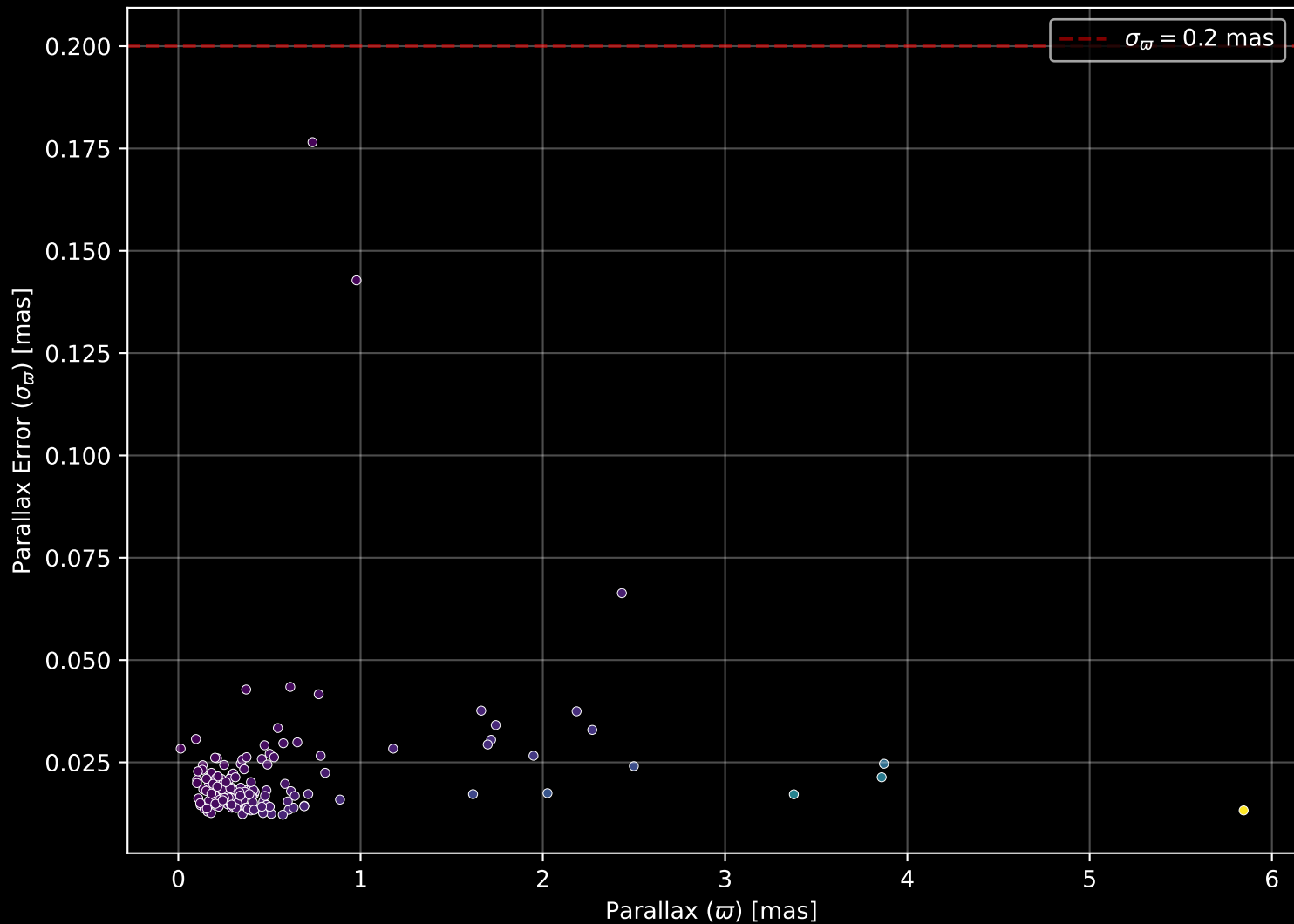
APOGEE DR17 Field: [229+04] Parallax Quality (n= 160)
