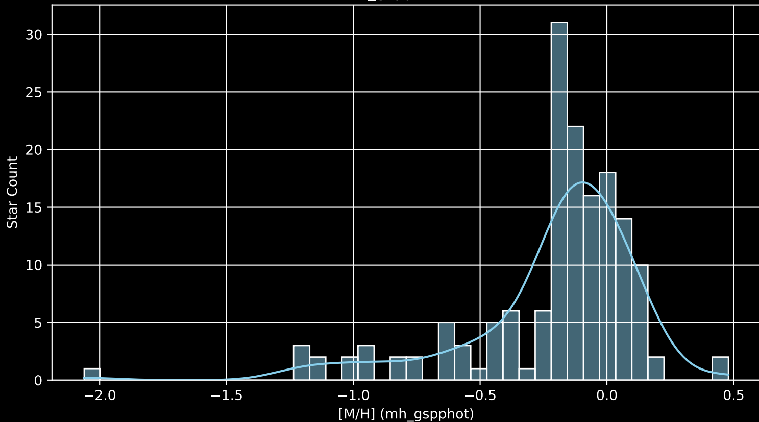
APOGEE DR17 Field: [229+04 [M/H] (mh_gspphot) (n= 157)
