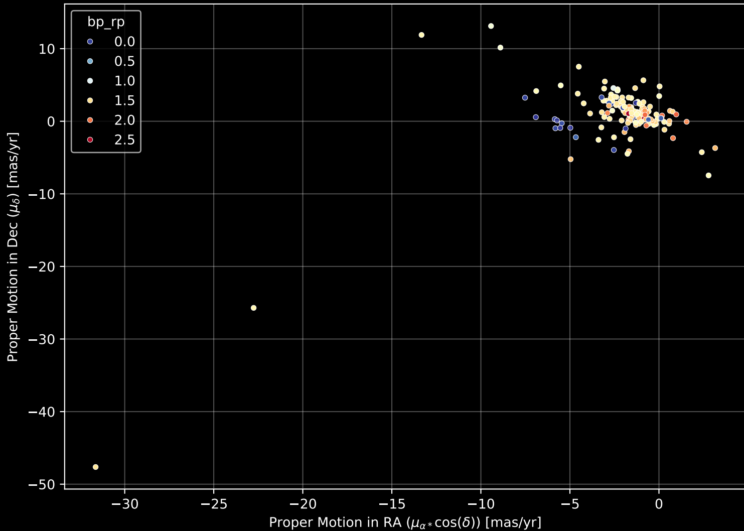
APOGEE DR17 Field: [229+04] Proper Motion Diagram (n= 160)
